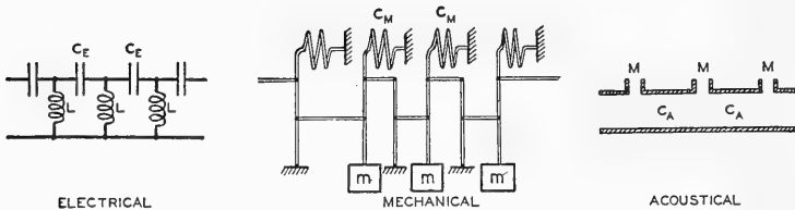
FIG. 4.10. High pass wave filters. (Courtesy of The Blakiston Company from Olson and Massa, "Applied Acoustics.")
